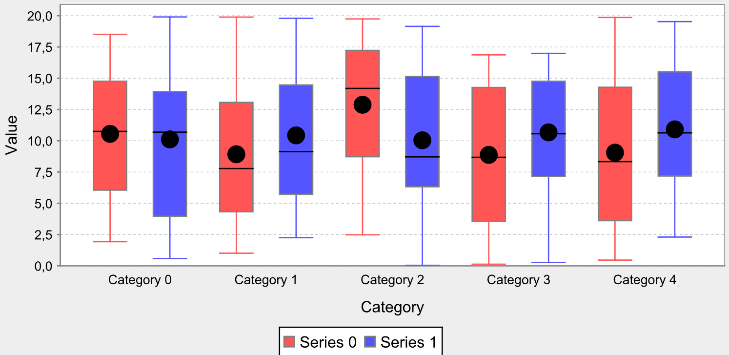
Box and Whisker chart
