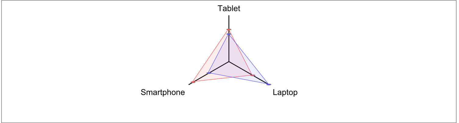
Spider chart
